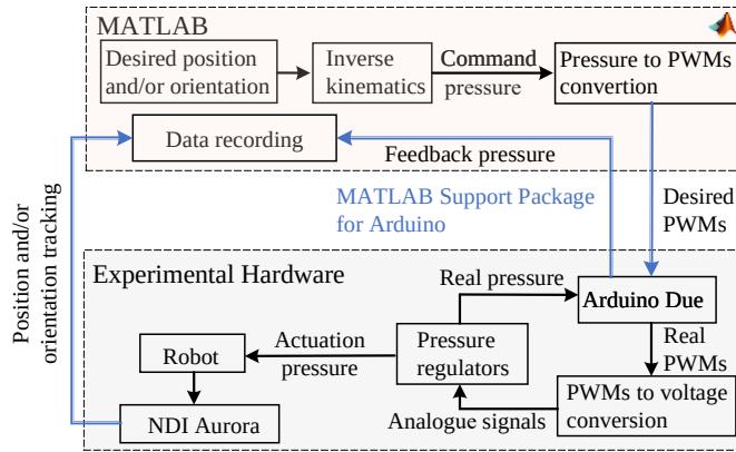
Fig. S1. Scheme for inverse kinematics control. MATLAB and the Arduino board communicate via the MATLAB Support Package for Arduino.
