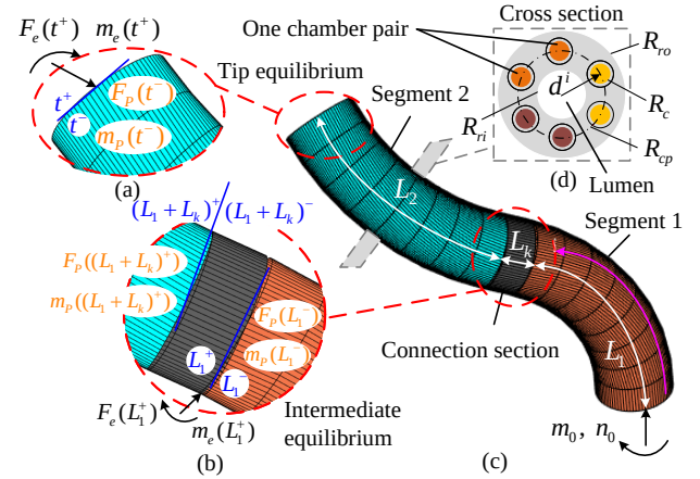
Fig. 1. Illustration of a two-segment robot: (a) Tip equilibrium at the tip of Segment 2. (b) Intermediate equilibrium at the tip of Segment 1. (c) Segment 1 (bottom module) and Segment 2 (top module). (d) Cross-sectional view. Three chamber pairs are distributed evenly with an angle of 120^\circ .
