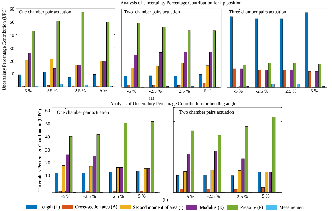
Fig. S3. Analysis of uncertainty percentage contribution with regards to the (a) tip position and (b) tip bending angle, where uncertainties in the robot length, cross-sectional area, second moment of area, modulus, actuation pressure and sensor measurement are included.
