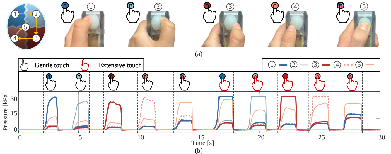
Fig. 5. Touching-sensing capabilities of the multi-cavity soft button. (a) Sequence of touches to the soft button, starting with the dark blue in the top left and proceeding clockwise around the surface to stimulate each cavity on the first layer. The touch sequence finishes by pressing the centre cavity. (b) Relative pressure for each stimulated cavity, touched with the gentle touch and the extensive touch.
