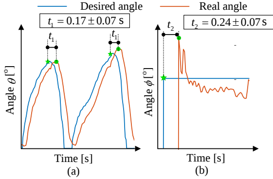
Fig. 11. Results for Experiment 1: Time delay analysis of (a) the bending angle \theta and (b) the out-of-plane angle \phi . The time delay is defined as the difference in time between the peaks of the desired angle (green star) and the actual angle (green circle), denoted by t_1 and t_2 .
