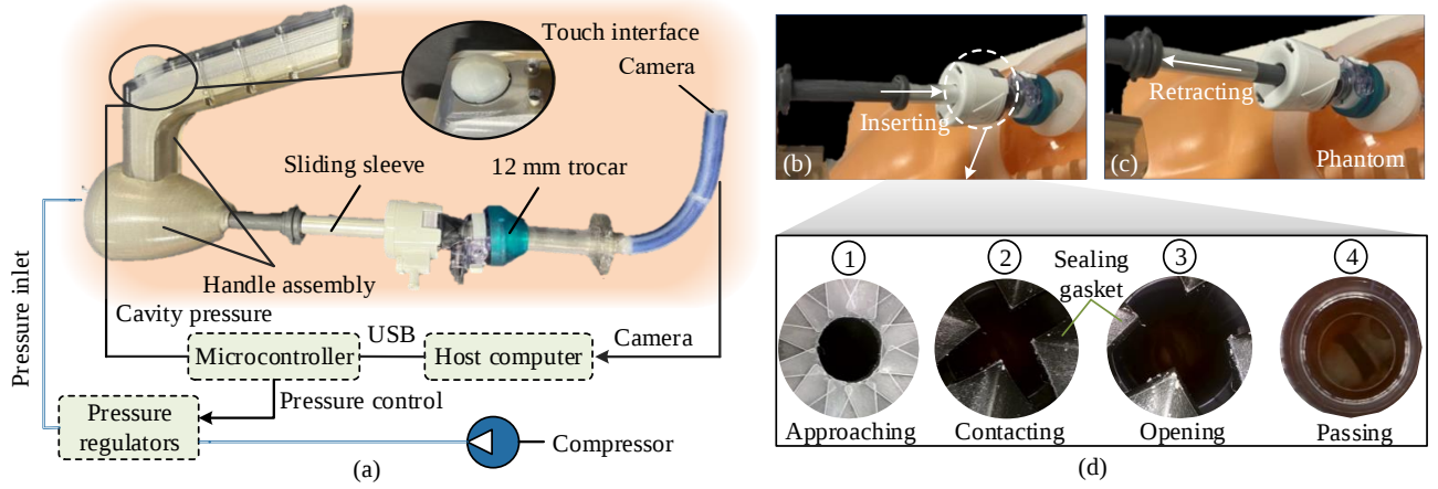
Fig. 4. (a) Assembly of the handheld soft robotic laparoscopy device with a multi-cavity touch interface. Operating the device in a phantom environment, when (b) inserting and (c) retracting the sliding sleeve. (d) The camera view when inserting the soft robotic device to a 12 mm trocar port.
